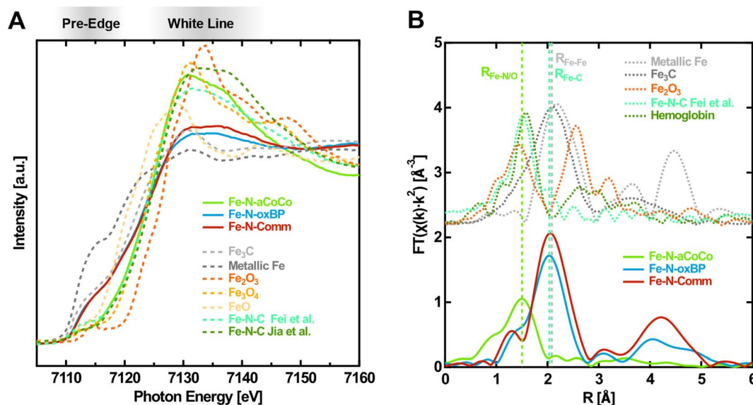
Fig. 1 Fingerprinting at the Fe K-edge of the Fe–N–C catalysts in the oxidized state (1.0 V vs. RHE applied). (A) XANES-region of the Fe K-edge with references of iron carbide 29 ( \text{Fe}_3\text{C} ), metallic iron, iron oxides 30 ( \text{Fe}_2\text{O}_3 , \text{Fe}_3\text{O}_4 , and \text{FeO} ) and different Fe–N–C materials (from Fei et al. 28 and Jia et al. 27 ). (B) Fourier transform of the EXAFS-region with references of iron carbide 29 ( \text{Fe}_3\text{C} ), metallic iron, iron oxide 23 ( \text{Fe}_2\text{O}_3 ) and an exemplary Fe–N–C material from Fei et al. 28 and glycated hemoglobin. 31
