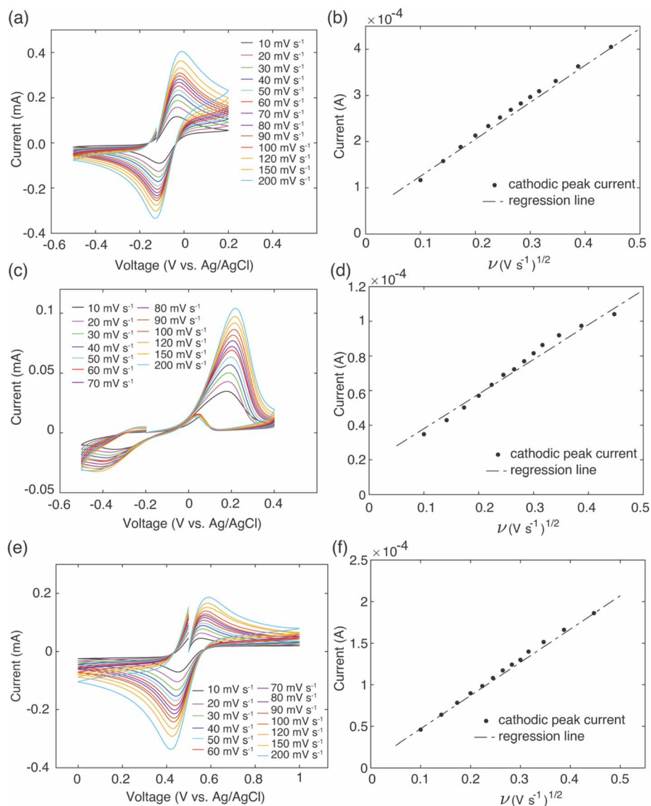
Fig. 8 Cyclic voltammograms at scan rates from 10 \text{mV s}^{-1} to 200 \text{mV s}^{-1} using brine solutions containing only added Fe 2+ /Fe 3+ (chlorides) or the Fe with additional ligands. The mediator concentration was 0.1 M for all cases, and the mediators used were (a) EDTA-Fe 2+ , (c) citrate-Fe 2+ , and (e) Fe 2+ /Fe 3+ chloride. The total Fe concentration in each brine solution was equimolar of Fe 2+ and Fe 3+ . Cathodic peak currents as a function of square root of scan rate determined from the CV scans are also shown for (b) EDTA-Fe 2+ , (d) citrate-Fe 2+ , and (f) Fe 2+ .
