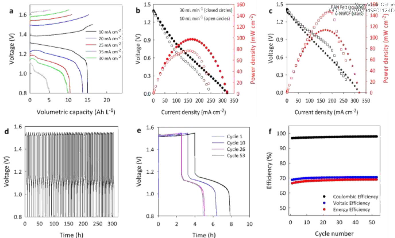
Fig. 6 Electrochemical performance of RFBs with NWCF in zinc iodide. a) Charge-discharge curves at 30 \text{ mL min}^{-1} , b) Polarization curves at varying flowrates, c) Polarization curves at 30 \text{ mL min}^{-1} for RFBs with \text{KMnO}_4 -treated NWCF electrodes and PAN-derived carbon felt electrodes, d-f) Cycling performance at 25 \text{ mA cm}^{-2} and 60 \text{ mL min}^{-1} .
