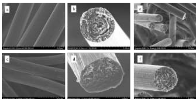
Fig. 2 SEM micrographs of (a, b) non-woven pitch-based carbon fibers, (c, d) commercial PAN-derived carbon felt, (e, f) \text{KMnO}_4 treated non-woven pitch-based carbon fibers.
