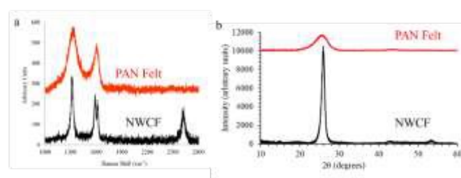
Fig. 3 (a) Raman Spectra and (b) X-ray diffractogram of PAN-derived carbon felt and NWCF electrodes.
