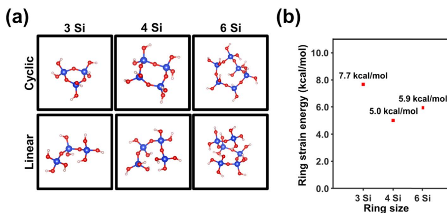
Fig. 2 (a) DFT optimized structures of systems involving n -membered-tetrahedral SiO 2 rings/chains with n = 3, 4 and 6. (b) Variation of the strain energy with the size of the ring.
