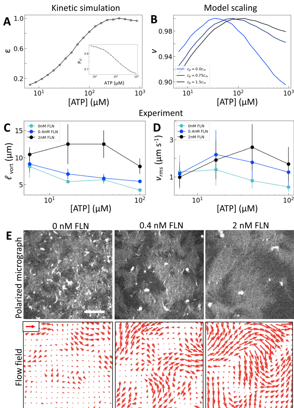
Fig. 4 Microscopic crosslinking alters nematic energy distribution. (A) Normalized \varepsilon and P_{cl} (inset) calculated for trimeric motors. (B) Normalized v from model scaling. (C and D) v_{rms} and \ell_{vort} measured for trimeric driven nematics with filamin (FLN) added as indicated. (E) Polarized fluorescence micrographs (gray, top row) with corresponding flow fields (red arrows, bottom row) for trimeric motors at 100 \mu\text{M} ATP with FLN added as indicated. Scale arrow is 3 \mu\text{m s}^{-1} . As above, error bars for speed are standard deviations over 100 s of steady-state activity. Error bars for length scale are standard deviations on five sets of five non-overlapping frames from a single experiment.
