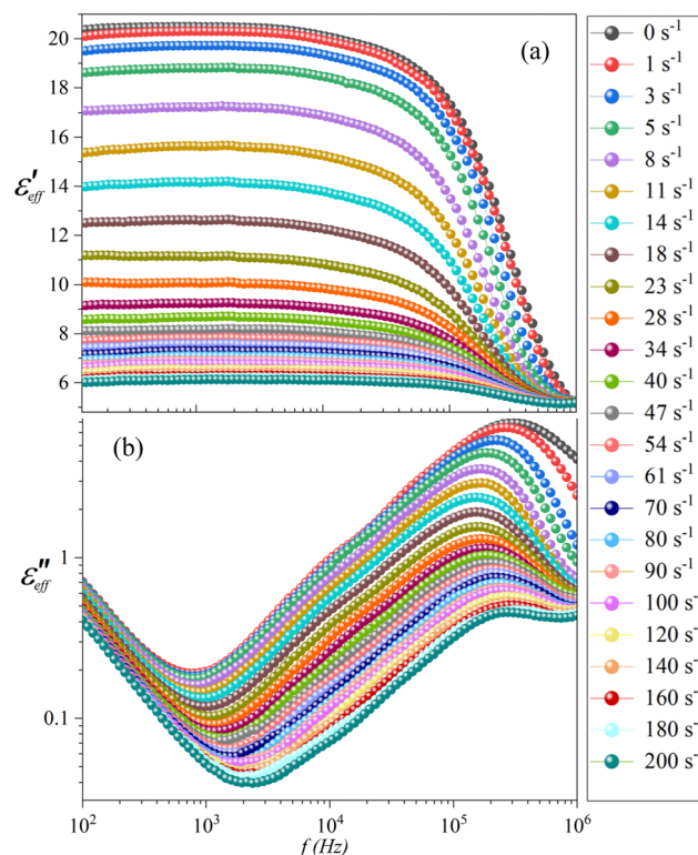
Fig. 2 Plots of (a) real ( \varepsilon'_{\text{eff}} ) and (b) imaginary ( \varepsilon''_{\text{eff}} ) components of the effective dielectric constant with frequency f , at different shear rates. Note that the magnitude of the AC probe voltage is 20 V, which is much higher than the Fredericksz threshold voltage ( V_{\text{th}} = 0.9 \text{ V} ). Measurements are made at temperature T = 5 \text{ °C} .
