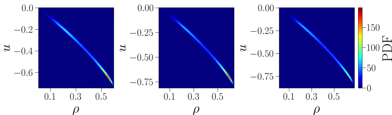
Fig. 4 Joint probability density functions of energy density u and particle density \rho at the critical point for u_{EE} = u_{PP} = 0.0 and three different values of \gamma = 30, 40, 50 from left to right.
