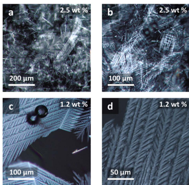
Fig. 25 The feather-like aggregates of SDS in the ChCl–Gly eutectogel from PLM. Magnification 10 \times (a), 20 \times (b and c), and 40 \times (d). Reproduced from L. Matthews, S. Ruscigno, S. E. Rogers, P. Bartlett, A. J. Johnson, R. Sochon and W. H. Briscoe, Fracto-eutectogels: SDS fractal dendrites via counterion condensation in a deep eutectic solvent, Phys. Chem. Chem. Phys. , 2021, 23 , 11672–11683 with permission from the PCCP Owner Societies, under a Creative Commons Attribution 3.0 Unported License.
