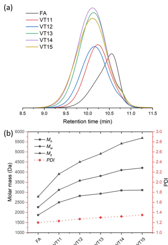
Fig. 1 Modification of commercially available FA with PG and GA: (a) SEC chromatograms (RI detector) in 0.067 \text{ mol l}^{-1} \text{ Na}_2\text{HPO}_4 in bidistilled- \text{H}_2\text{O} ; (b) number-average molecular weight ( M_n ), weight-average molecular weight ( M_w ), size-average molecular weight ( M_z ) and dispersity index ( \text{PDI} = M_w/M_n ).
