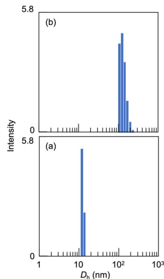
Fig. 18 The number conversion distributions in light scattering: (a) the isolated polymer at SDS/AA = 0.01 and (b) aggregates at SDS/AA = 0.1. M_w = 15\,000 , [AA]_0 = 3.59 \times 10^{-3} \text{ mol L}^{-1} .
