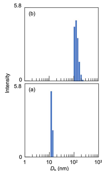
Fig. 18 The number conversion distributions in light scattering: (a) the isolated polymer at SDS/AA = 0.01 and (b) aggregates at SDS/AA = 0.1. M_w = 15\,000 , [AA]_0 = 3.59 \times 10^{-3} \text{ mol L}^{-1} .
