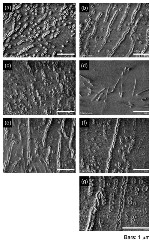
Fig. 22 FE-SEM images of the aggregate morphologies for the polymer surfactants with the molecular weight: (a and b) M_w = 15\,000 , (c and d) 5000 and (e–g) 1600. (a, c and e) [AA]_0 = 3.42 \times 10^{-3} \text{ mol L}^{-1} and (b, d, f and g) 1.03 \times 10^{-2} \text{ mol L}^{-1} .
