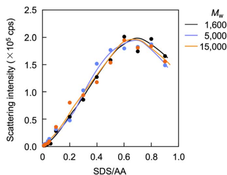
Fig. 19 Variation in scattering intensity of the polymer solution versus the SDS/AA ratio. [AA]_0 = 3.59 \times 10^{-3} \text{ mol L}^{-1} .
