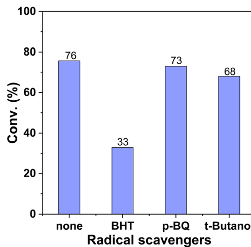
Fig. 6 Control experiments with different radical scavengers.
