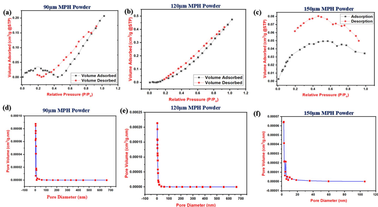
Fig. 2 (a–c) BET adsorption–desorption isotherms for 90\text{ }\mu\text{m} , 120\text{ }\mu\text{m} and 150\text{ }\mu\text{m} MPH powder respectively and (d–f) BJH pore size analysis of 90\text{ }\mu\text{m} , 120\text{ }\mu\text{m} and 150\text{ }\mu\text{m} MPH powder respectively.
