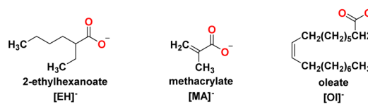
Fig. 3 Carboxylate anions used in this work.
