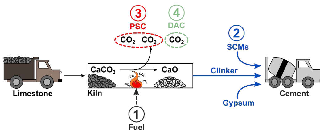
Figure 1. Schematic of the cement production outlining the key process steps and retrofit decarbonization options that we will discuss in this work. The CO 2 emissions associated with this process can come from process emissions from the calcination of limestone (CaCO 3 ) to lime (CaO) and fuel consumption. In this work, we consider mitigating these emissions by evaluating the costs of 1) alternative fuels, 2) clinker
