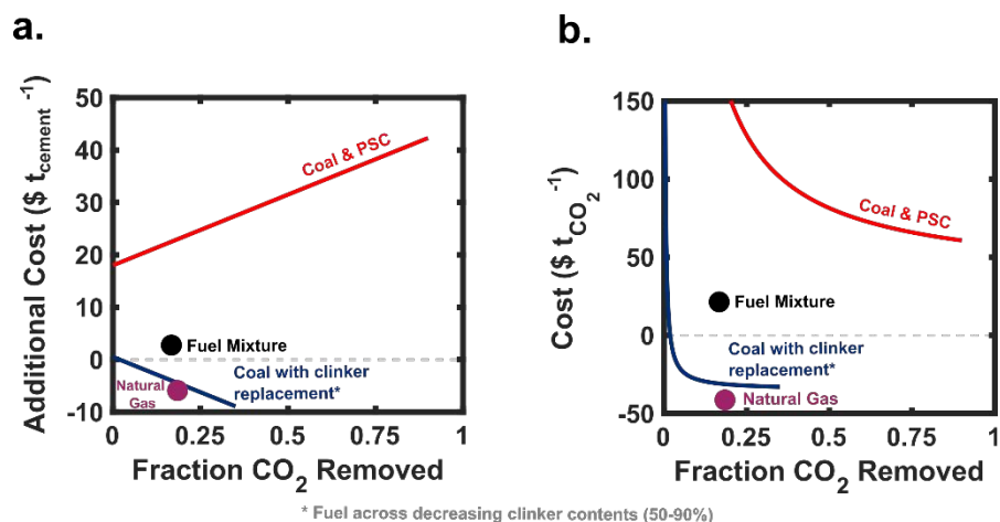
Figure 2. (a) Additional costs of implementing the decarbonization technology for cement production ( \$ t_{\text{cement}}^{-1} ) beyond the current baseline costs of cement production ( \$106 t_{\text{cement}}^{-1} ). (b) Costs of \text{CO}_2 removal ( \$ t_{\text{CO}_2}^{-1} ) associated with pursuing clinker replacement, fuel replacement, and/or retrofitting a capture unit onto the plant with varying costs of capture. The costs of capture at the maximum capture fraction of 90% are \$60 t_{\text{CO}_2}^{-1} , in-line with current PSC systems. The fuel alternatives are single data points because the technology can only remove a set amount of \text{CO}_2 when the fuel is replaced. On the contrary, the clinker replacement and PSC curves represent the range of decarbonization amounts that can result by varying the amount of clinker replaced or \text{CO}_2 captured, respectively. The dashed gray line at \$0 in both figures represents the baseline costs.
