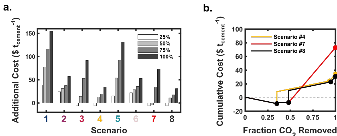
Figure 4. (a) Additional costs to a cement plant ( \$ \text{ t}_{\text{cement}}^{-1} ) to achieve up to net-zero \text{CO}_2 removal assuming PSC = \$60 \text{ t}_{\text{CO}_2}^{-1} and DAC = \$200 \text{ t}_{\text{CO}_2}^{-1} . The costs at 25%, 50%, 75%, and 100% removal are representative of actual costs that will be incurred by the cement manufacturing facility to achieve the desired \text{CO}_2 removal. (b) The total additional costs to a cement plant ( \$ \text{ t}_{\text{cement}}^{-1} ) to achieve a fraction of \text{CO}_2 removal in Scenarios #4, #7, and #8. The dashed gray line at \$0 \text{ t}_{\text{cement}}^{-1} represents the baseline costs.
