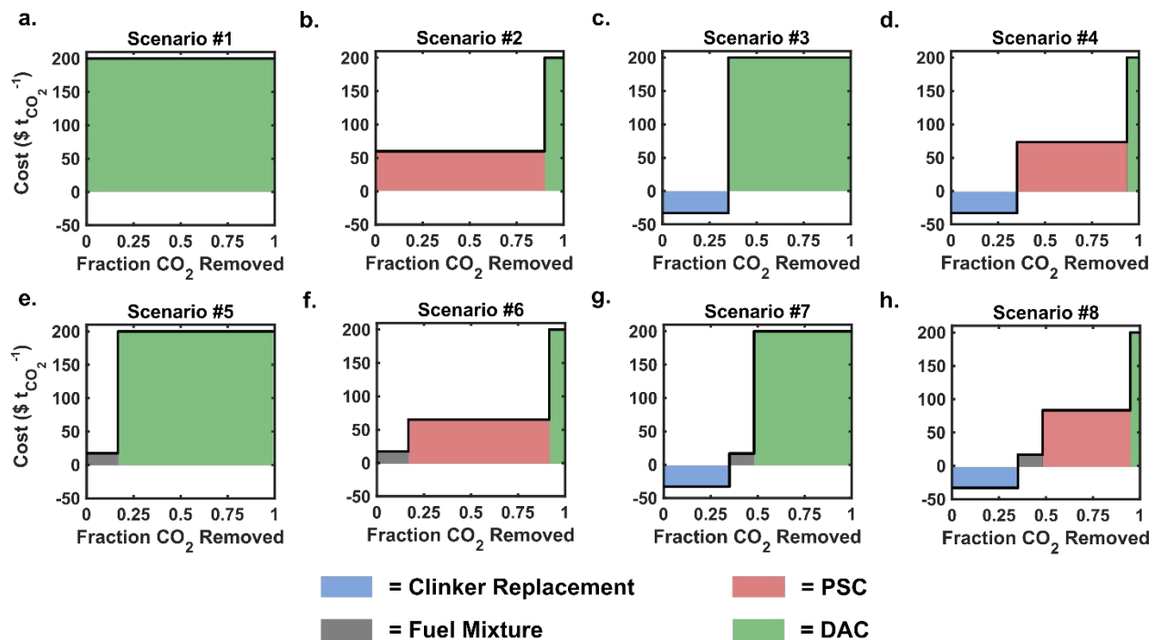
Figure 3. Dispatch curve of technologies for each of the decarbonization pathways outlined in Table 1 (a – h). Dispatch curve is developed based on the costs of CO 2 removal ( \$ t_{\text{CO}_2}^{-1} ). The black line indicates the costs associated with decarbonizing via the technology associated with the color under/above the curve.
