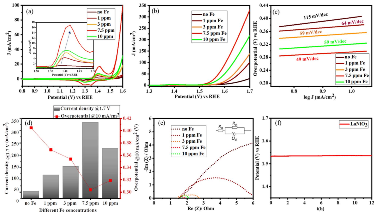
Fig. 4 (a) Cyclic voltammograms after 50 cycles. The inset shows the shift in the oxidation peak of Ni in the presence of different Fe contents. (b) Linear sweep voltammograms (LSV) after 100 cycles of CV (c) Tafel plots (d) overview on the overpotential at 10 \text{ mA cm}^{-2} and current density at 1.7 \text{ V} vs. RHE (e) Nyquist plots from EIS measurements at 1.66 \text{ V} vs. RHE on \text{LaNiO}_3 in different concentrations of Fe in the electrolyte (1 M KOH) and (f) chronopotentiometry on \text{LaNiO}_3 at 10 \text{ mA cm}^{-2} for 12 h in 1 M KOH with 7.5 ppm of Fe impurity.
