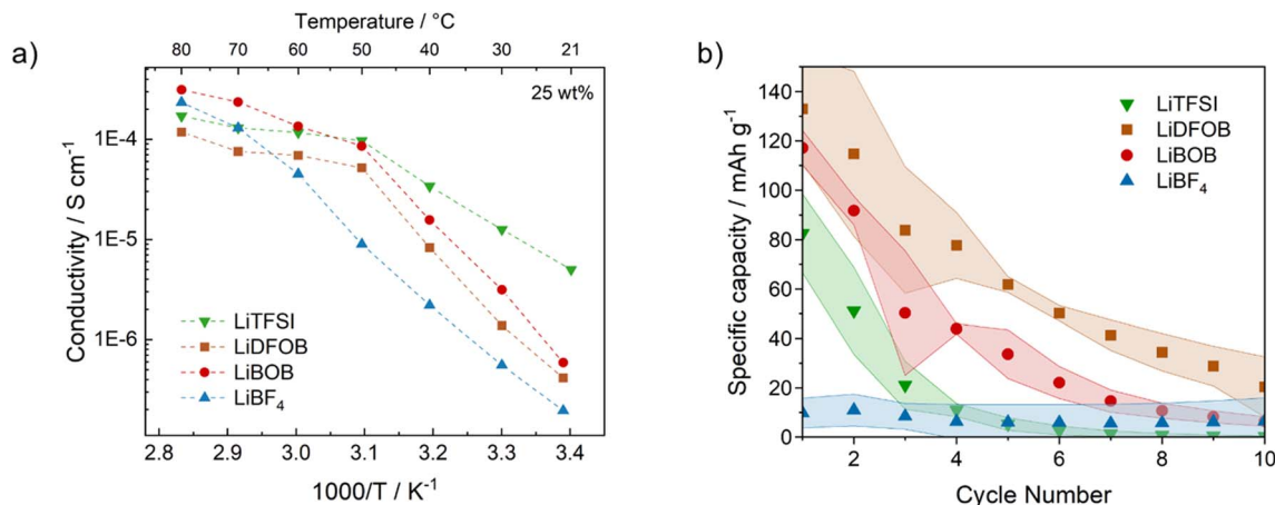
Fig. 2 (a) Ionic conductivity as a function of temperature of PEO:salt SPEs, salt concentration fixed at 25 wt%. (b) Specific capacity of anode-free batteries (Cu vs. LFP, N/P = 0) containing different PEO:salt SPEs. Test performed at 60 °C, 0.1C ( \approx 40 \mu\text{A cm}^{-2} ), in the voltage interval 2.7–4.0 V.
