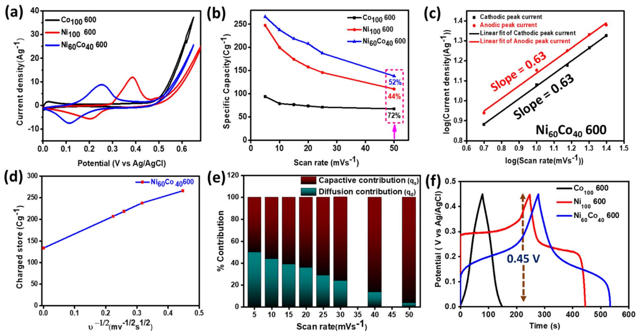
Fig. 5 (a) CV curves, (b) plot of C_s vs. scan rate for activated Ni_{100} 600, Co_{100} 600, and Ni_{60}Co_{40} 600 samples, (c) b value estimation (within the 5 to 25 mV s^{-1} scan rate range), (d) C_s vs. \nu^{-1/2} plot for activated Ni_{60}Co_{40} 600, (e) the bar diagram showing % contribution from diffusion and capacitive processes at 5 to 50 mV s^{-1} scan rates and (f) GCD curves for Ni_{100} 600, Co_{100} 600, and Ni_{60}Co_{40} 600 recorded at 1 A g^{-1} .
