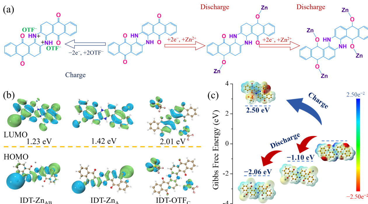
Fig. 4 (a) Mechanism illustration of the Zn//IDT battery with 2 M Zn(OTF)_2 electrolyte. (b) The calculated energy level of IDT associated with different amounts of Zn^{2+} and OTF^- . (c) Molecular ESP simulation and Gibbs free energy.
