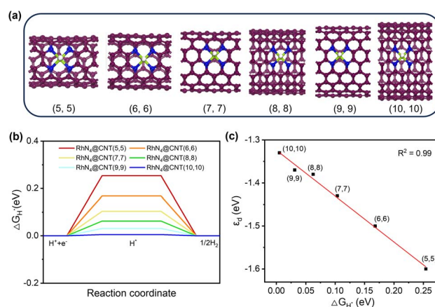
Fig. 3 HER activity of \text{RhN}_4\text{@CNT} s with six different curvatures. (a) Optimized geometric model of \text{RhN}_4\text{@CNT}(n, n) ( n = 5\text{--}10 ) adsorbed with a single H atom. (b) \Delta G_{H^*} on \text{RhN}_4\text{@CNT}(n, n) ( n = 5\text{--}10 ). (c) Correlation between \Delta G_{H^*} and d-band center ( \varepsilon_d ) of Rh anchored on CNTs with different nanotube diameters.
