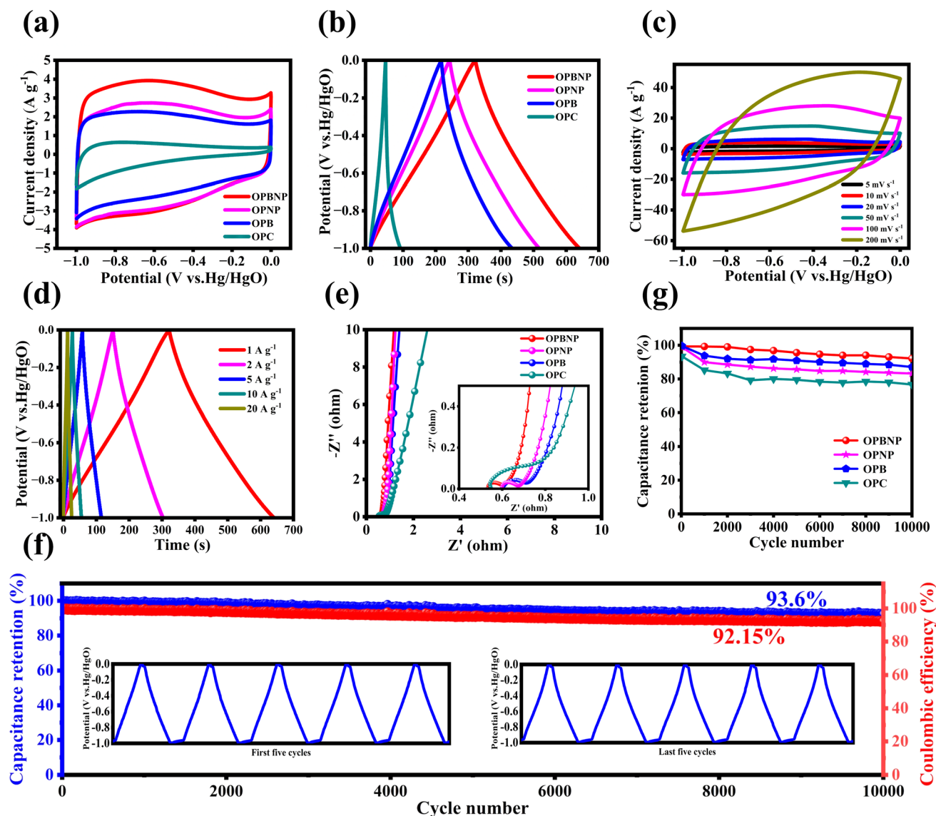
Fig. 3 Electrochemical performance of OPC, OPB, OPNP and OPBNP for supercapacitor in three-electrode system in 6 M KOH. (a) CV curves at 10 mV s -1 ; (b) GCD curve at 1 A g -1 ; (c) CV and (d) GCD curves of OPBNP at different scan rates and current densities; (e) EIS spectroscopy (inset: equivalent circuit diagram); (f) cycling performances at 5 A g -1 of OPBNP (inset: GCD curves of the first and last five cycles); and (g) comparison chart of cycling performance of four samples.
