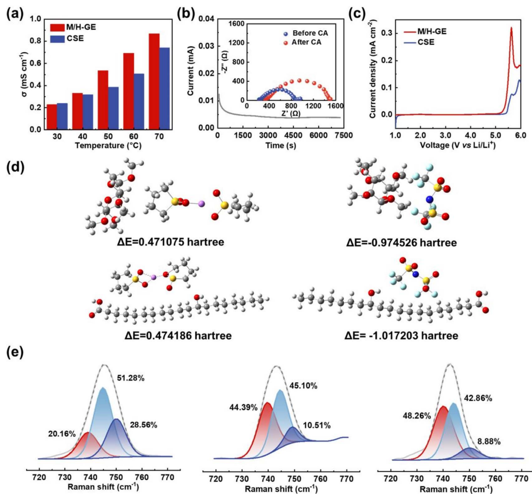
Fig. 5 Li + conduction properties and mechanism of GEs: (a) EIS results of stainless steel symmetric cells using the M/H-GE membrane tested at 30–70 °C. (b) Direct current (DC) polarization of the Li||M/H-GE||Li cell at 10 mV (inset: EIS spectra before and after DC polarization). (c) LSV curves of the Li||M/H-GE||stainless steel cell and Li||CSE||stainless steel cell. (d) Simulated gelator–[Li(SL) 2 ] + complex cation interactions and gelator–TFSI - interactions. (e) Raman spectra of CSE, H-GE, M/H-GE membrane.
