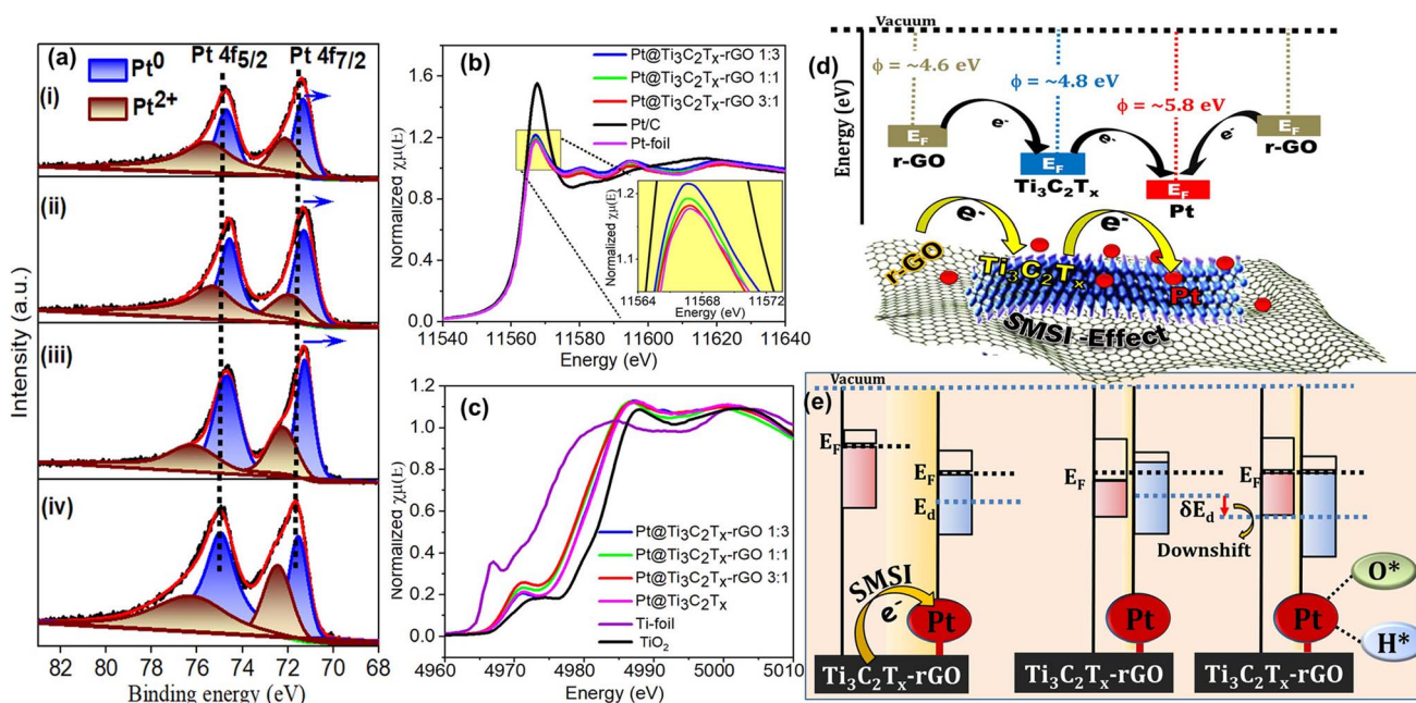
Fig. 7 (a) XPS of the Pt 4f region of (i) Pt@Ti 3 C 2 T x -rGO 1 : 3, (ii) Pt@Ti 3 C 2 T x -rGO 1 : 1, (iii) Pt@Ti 3 C 2 T x -rGO 3 : 1 and (iv) Pt/C. Normalized XANES at (b) the Pt L 3 edge and (c) the Ti K-edge for all the developed catalysts along with the control samples (Pt-foil, Pt/C, Ti-foil and TiO 2 ). (d) Schematic illustration of the charge transfer mechanism facilitated by the difference in work function ( \phi ) between Pt and the Ti 3 C 2 T x -rGO support. (e) Illustration of charge transfer induced downshift in the Pt d-band of the Pt@Ti 3 C 2 T x -rGO catalyst.
