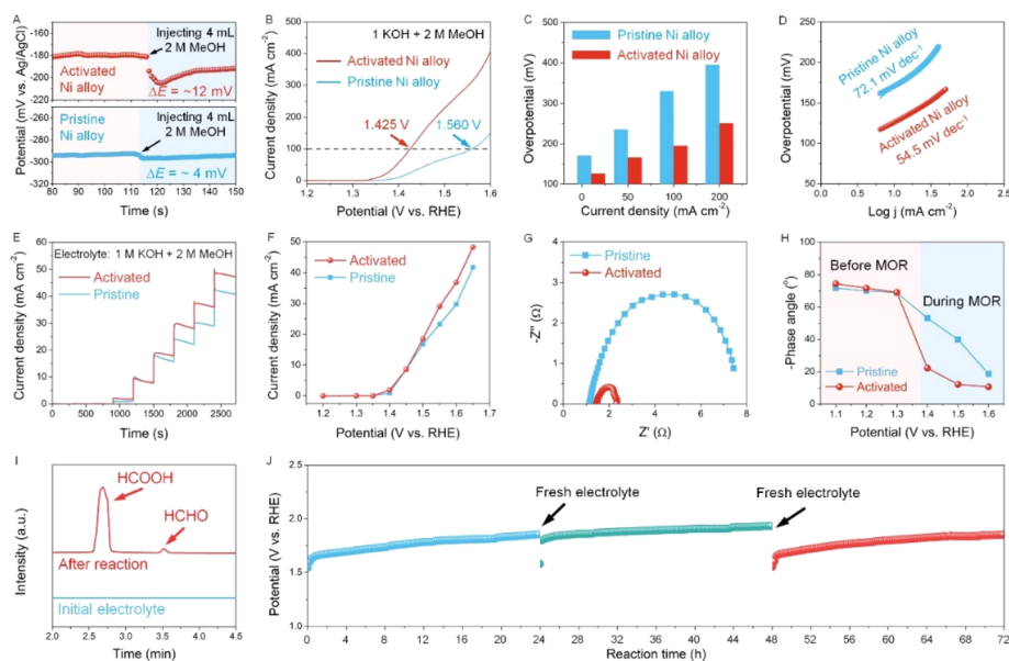
Fig. 3 (A) OCP test of pristine and activated Ni alloys before and after injecting 4 mL 2 M MeOH. (B) LSV curves (with 90% iR -correction) of pristine and activated Ni alloys in 1 M KOH + 2 M MeOH at 5 mV s -1 . (C) Overpotential comparison at different current densities. (D) Corresponding Tafel plots. (E) j - t curves of pristine and activated Ni alloys at different potentials using NPV. (F) The corresponding NPV of pristine and activated Ni alloys. (G) Nyquist plots of pristine and activated Ni alloys at 1.5 V RHE . (H) Phase angles obtained from EIS spectra recorded at different potentials. (I) HPLC profiles of products before and after the electrooxidation reaction over the activated Ni alloy in electrolyte containing 1 M KOH + 2 M MeOH. (J) Chronopotentiometry test of the activated Ni alloy in 1 M KOH + 2 M MeOH without iR -correction.
