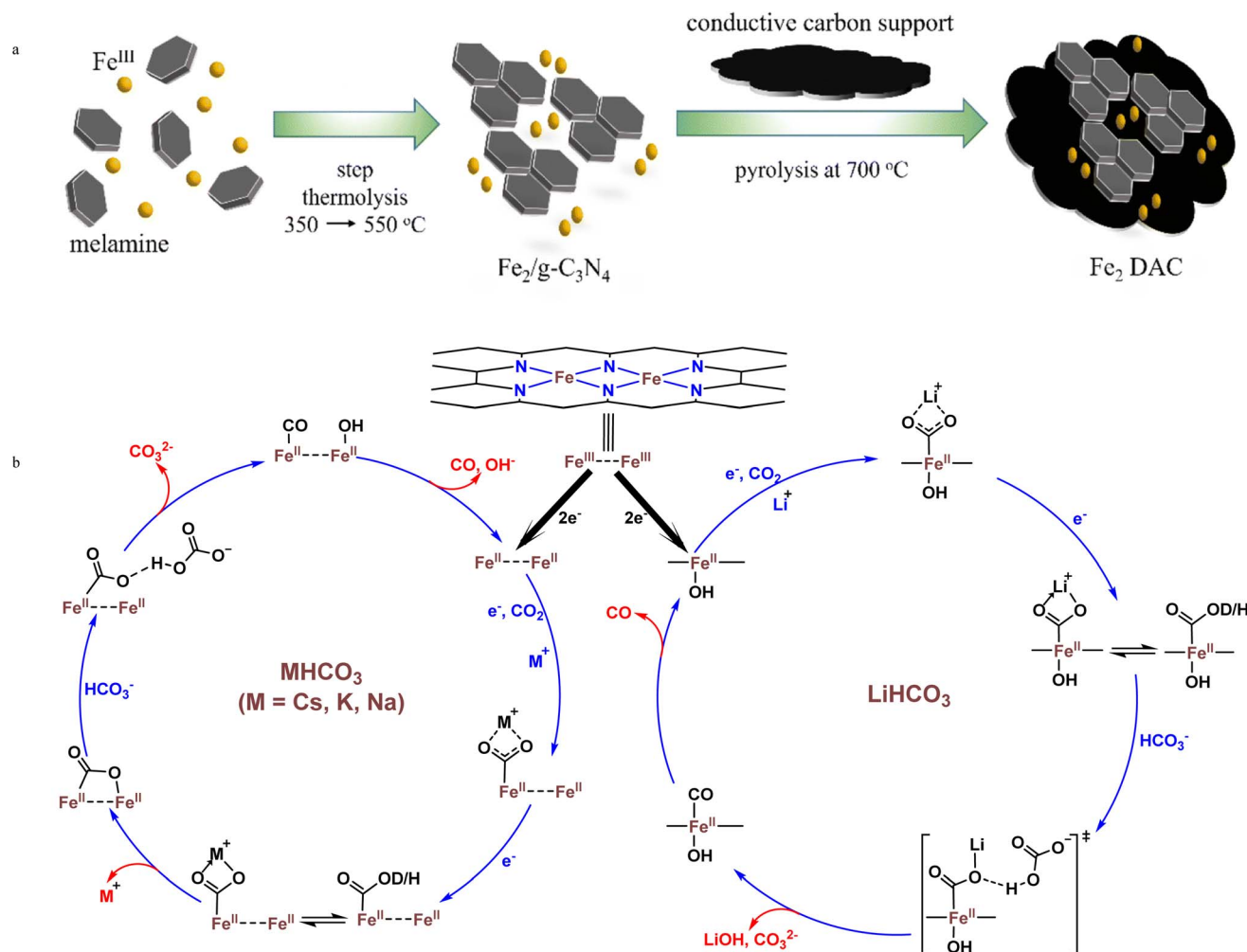
Fig. 7 (a) Synthetic scheme of an atomically precise dual \text{Fe}_2 catalyst ( \text{Fe}_2\text{DAC} ) using the di-nuclear \text{Fe}_2 site preservation strategy. 86 (b) \text{eCO}_2\text{RR} mechanism for \text{Fe}_2\text{DAC} involving alkali metal bicarbonates.
