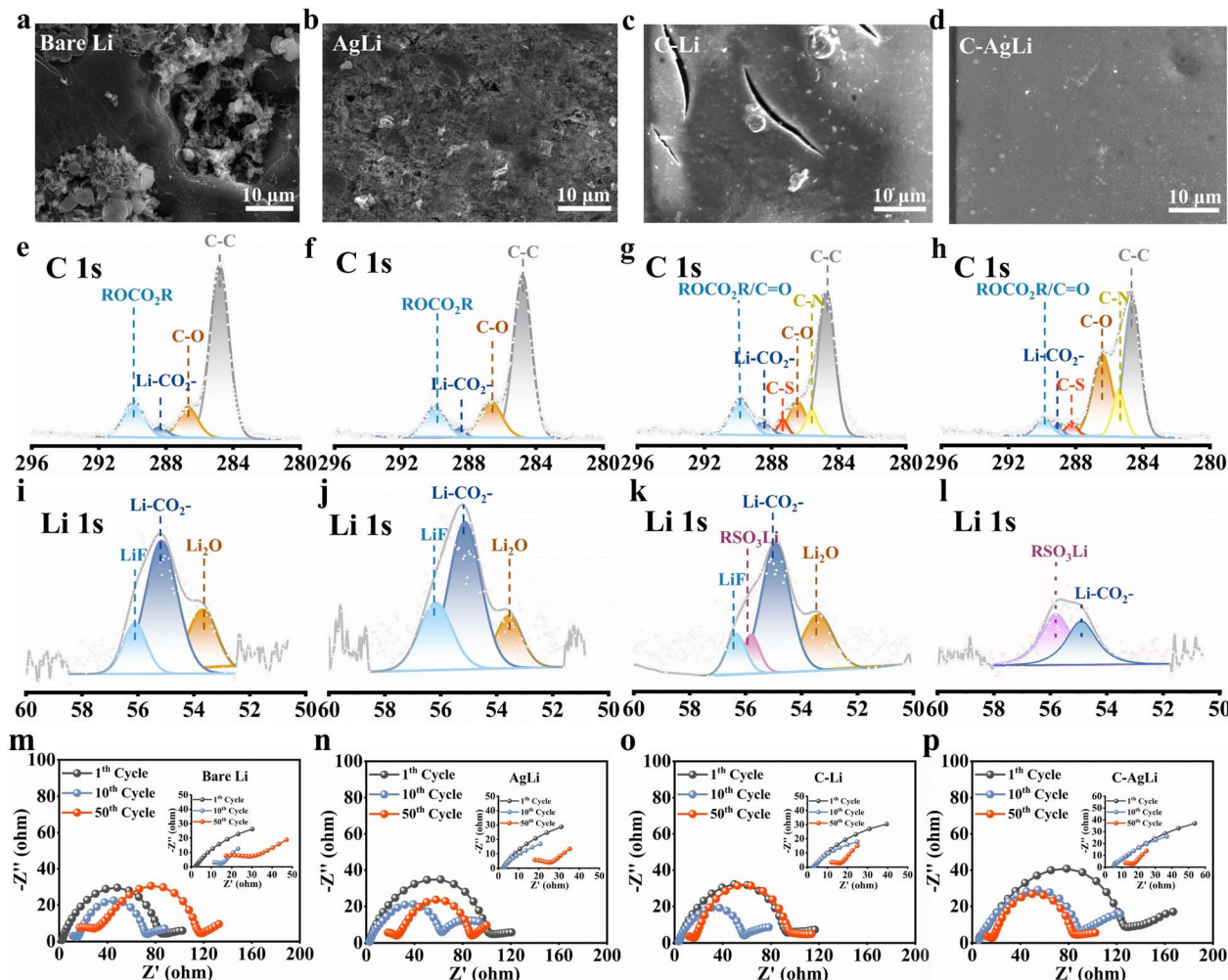
Fig. 4 Comparison for morphologies, components, and EIS of lithium metal anodes based on different substrates after 50 cycles. Detailed SEM images of (a) bare Li, (b) AgLi, (c) C-Li, and (d) C-AgLi electrode after Li deposition; XPS spectra for the (e, f, g and h) C 1s and (i, j, k and l) Li 1s of the (e and i) bare Li, (f and j) AgLi, (g and k) C-Li, and (h and l) C-AgLi electrode, respectively. EIS spectra of symmetric cells with different substrates as working electrode after 1st, 10th and 50th cycles: (m) bare Li, (n) AgLi, (o) C-Li, and (p) C-AgLi. The capacities of Li deposition are 2 \text{ mA h cm}^{-2} .
