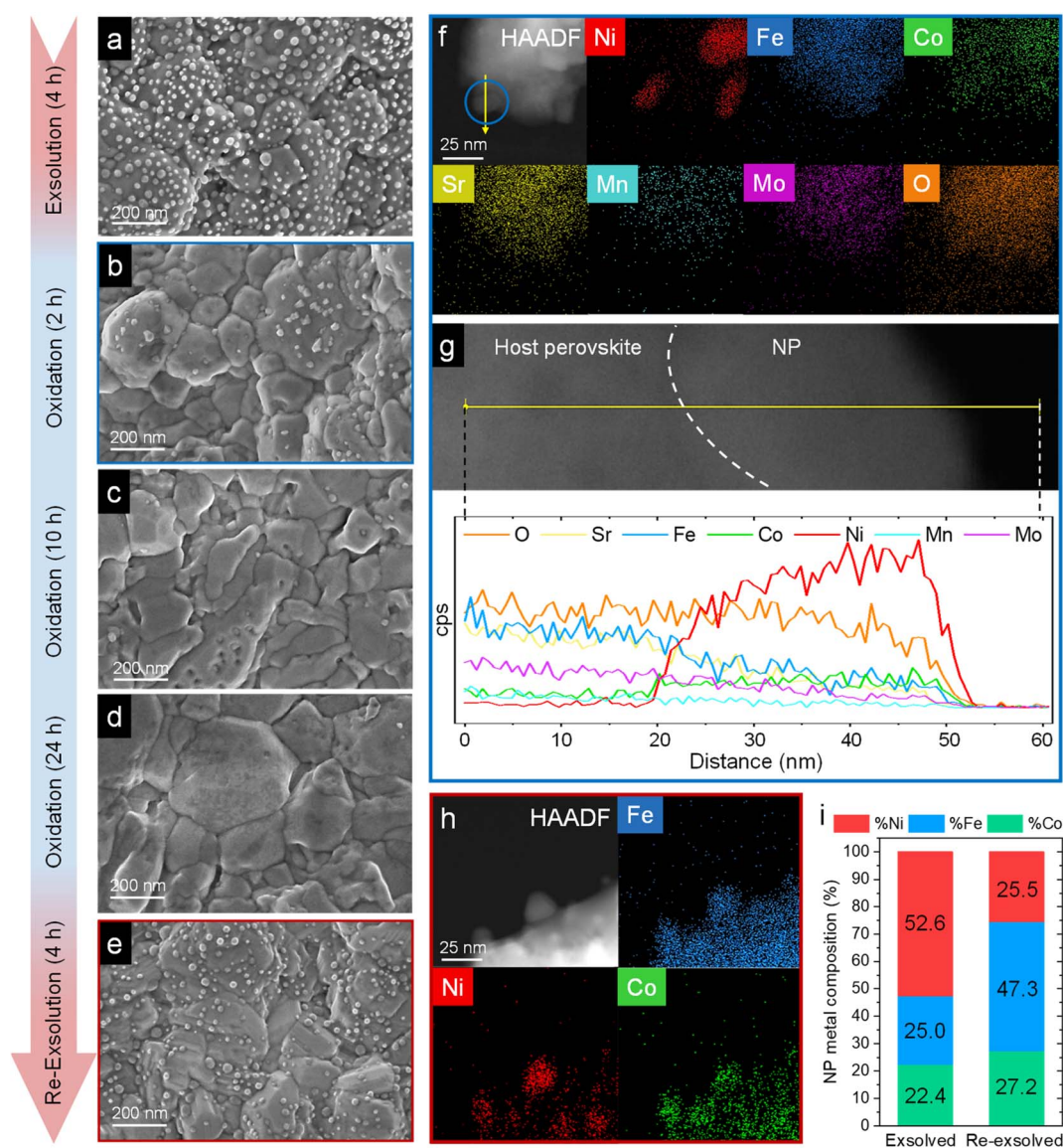
Fig. 11 HRFESEM micrographs of \text{Sr}_2\text{FeCo}_{0.2}\text{Ni}_{0.2}\text{Mn}_{0.1}\text{Mo}_{0.5}\text{O}_{6-\delta} after ex situ 800 °C, 4 h exsolution in 5% \text{H}_2/\text{Ar} flow (a). The same sample after re-oxidation at 800 °C in air for 2 (b), 10 (c), and 24 h (d). Following the 24 h re-oxidation, another reduction treatment (800 °C, 4 h, 5% \text{H}_2/\text{Ar} ) was performed for re-exsolution (e). HAADF and XEDS map images of the material after 2 h re-oxidation treatment (f) and line-scan analysis (yellow arrow) for one of the NPs, highlighted in blue (g). These compositional analyses reveal that, after re-oxidation, the remaining NPs are mainly composed of NiO. HAADF and map images of re-exsolved NPs, revealing that after re-exsolution ternary FeCoNi ternary alloys are also obtained (h). Compositional comparison of the exsolved NPs after first exsolution and re-exsolution (i). Compositional information of the first exsolution NPs were taken with permission from ref. 20.
