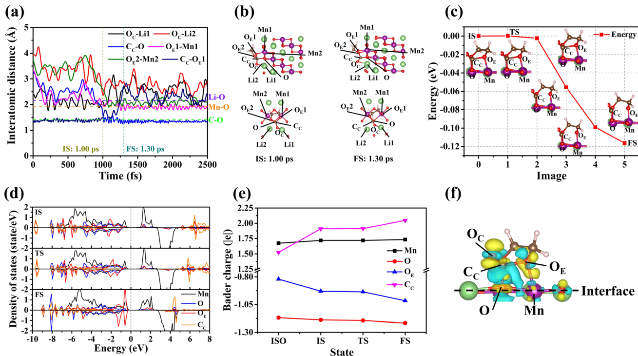
Fig. 3 (a) The changes in atomic distance upon decomposition of EC on the (10 \bar{1} ) surface. (b) and (c) The schematic diagram and energy barrier of EC decomposition on the (10 \bar{1} ) surface. (d) and (e) The PDOS and Bader charges of Mn, O, O E , and C C in different states. (f) The charge density difference between EC and the (10 \bar{1} ) surface after adsorption (the iso-surface charge density is assumed to be 5 \times 10^{-3} e \text{ bohr}^{-3} ).
