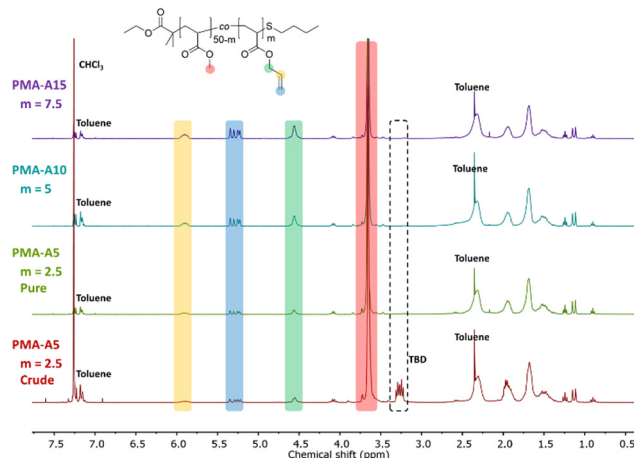
Fig. 1 1 H NMR spectra recorded in CDCl 3 of the crude PMA-A5 with observable TBD impurity at 3.25 ppm, and of all PMA-allyl polymers after treatment with Dowex 50 W X8.
