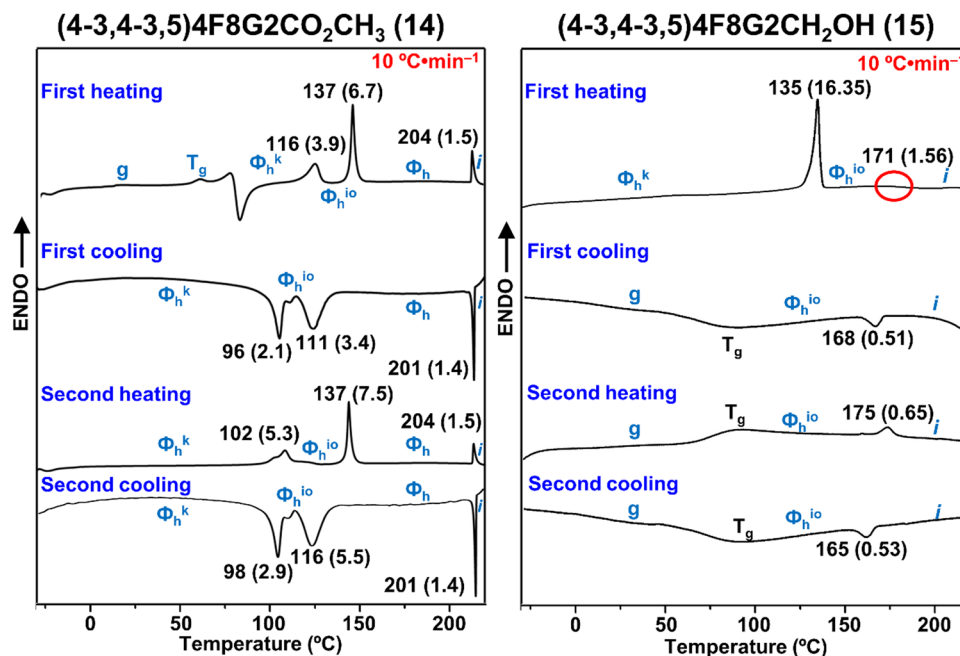
Fig. 1 DSC traces collected for (4-3,4-3,5)4F8G2 \text{CO}_2\text{CH}_3 (14) and (4-3,4-3,5)4F8G2 \text{CH}_2\text{OH} (15) at heating and cooling rate of 10\text{ }^\circ\text{C}\cdot\text{min}^{-1} . Phases determined by XRD, transition temperatures (in ^\circ\text{C} ), and associated enthalpy changes (in between parentheses in \text{kcal mol}^{-1} ) are indicated. \Phi_h^{\text{k}} , crystalline columnar hexagonal phase; \Phi_h^{\text{io}} , columnar hexagonal phase with intracolumnar order; \Phi_h , liquid crystalline columnar hexagonal phase; i, isotropic phase; g, glassy phase.
