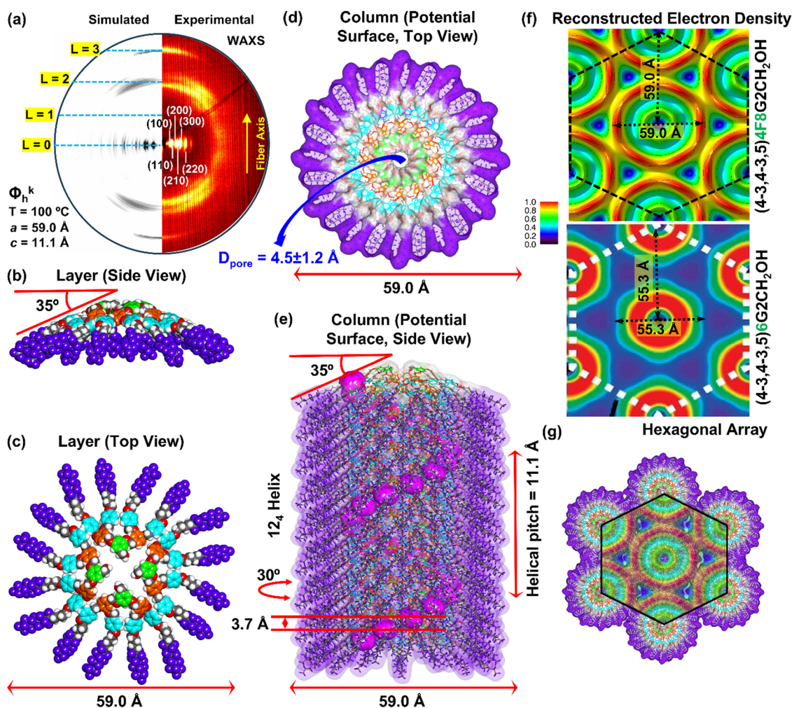
Fig. 6 X-ray diffraction analysis and molecular models of (4-3,4-3,5)4F8G2CH 2 OH (15) at 100 °C ( \Phi_h^k phase). (a) Wide-angle oriented fiber XRD patterns (WAXS) and simulated XRD patterns from the molecular model showing the similarity; (b) formation of the layer by four molecules showing the tilt angle (side view); (c) layer with four molecules (top view); (d) formation of the column by repeat of the tetramer layer (potential surface, side view); (e) column (potential surface, top view); (f) reconstructed relative electron density maps of the semifluorinated (4-3,4-3,5)4F8G2CH 2 OH (15) (top) and of the hydrogenated (4-3,4-3,5)6G2CH 2 OH (bottom) demonstrating the large difference between fluorinated and nonfluorinated structures as seen in the sharpness of microsegregation observed in the case of fluorinated chains; (g) hexagonal array by the columns (potential surface; top view). Color codes used in the molecular models are similar as shown in the ChemDraw structure of 15. O atoms, red; H atoms, white; F atoms, purple; C atoms in the phenyl rings connected apex -CH 2 OH group, green; C atoms in the phenyl rings connected of the first generation, orange; C atoms in other phenyl rings in the second generation, light blue; all other C atoms, grey. Potential surface is in fact the "van der Waals surface" and the color codes for the potential surface are similar as atom colors; transparency (50%) was added for clarity.
