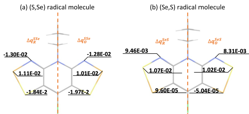
Fig. 3 Atomic Mulliken charge analysis of the neutral ( R^N ) and charged ( R^C ) geometries of (a) (S,Se) and (b) (Se,S) materials. In each image, the charge difference \Delta q for acceptor (A, reduction \Delta q_R^{XY} ) and donor (D, oxidation \Delta q_O^{XY} ) are shown in the half left and half right parts of the XY radical molecules, respectively, since the main changes between (S,Se) and (Se,S) systems are localized in N – E 2 – E 1 atoms. Note that \Delta q on the missing half of the molecules is equivalent to the one represented. See ESI,† Section S5 for the remaining systems.
