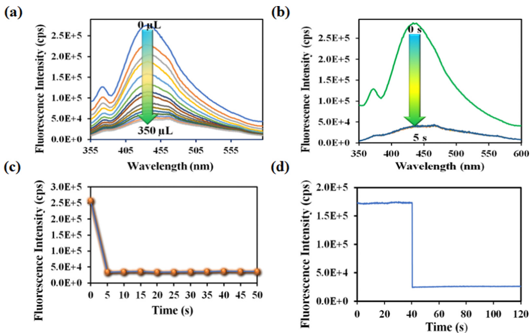
Fig. 6 (a) PL emission intensity plot for 1' with incrementally added nitenpyram. (b) Time-dependent PL emission intensity of 1' in 350 μL of 1 mM nitenpyram. (c) The PL emission intensity of the probe by changing the time after adding 350 μL, 1 mM nitenpyram. (d) Fluorescence kinetic study of the probe by recording the PL intensity at 430 nm by changing the time after the addition of 350 μL, 1 mM nitenpyram.
