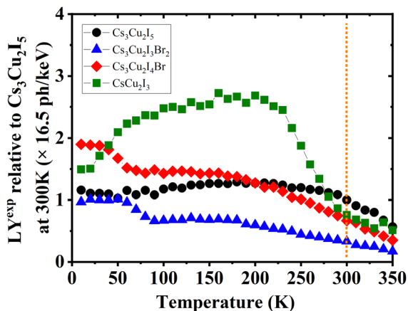
Fig. 6 Temperature-dependent experimental LY (LY exp ) spectra of Cs 3 Cu 2 I 5 , Cs 3 Cu 2 I 3 Br 2 , Cs 3 Cu 2 I 4 Br, and CsCu 2 I 3 , normalised to the LY of Cs 3 Cu 2 I 5 at 300 K derived using integrated RL intensities. The vertical dashed line indicates where the value of LY exp is taken using pulse height spectra at RT, see Fig. S13 (ESI†).
