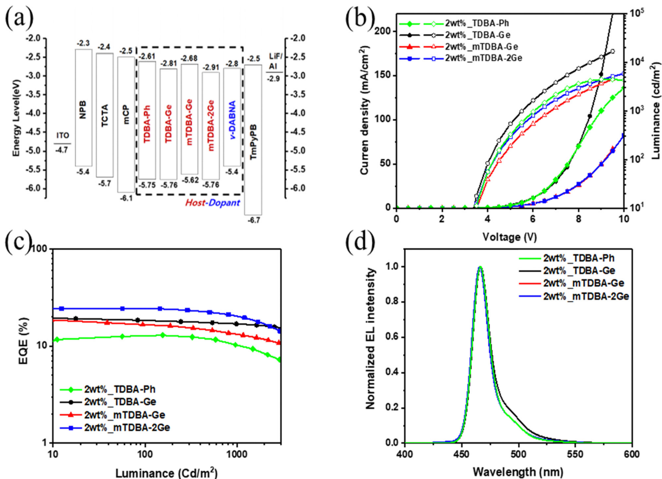
Fig. 4 OLED device performance of 2 wt% TDDBA-Ge , mTDDBA-Ge and mTDDBA-2Ge emitters: (a) energy-level diagram of doped OLED devices, (b) current–voltage–luminescence curve, (c) EQE–luminance curves and (d) EL spectra at 10 mA cm -2 .
