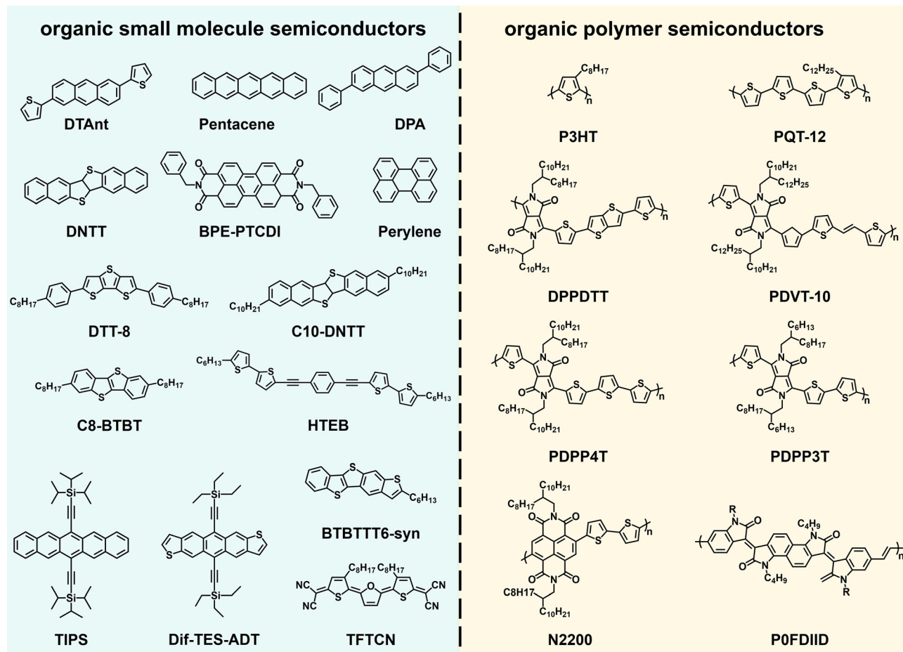
Fig. 2 Summary of organic small molecule semiconductors and organic polymer semiconductors for organic photonic synaptic transistors.
