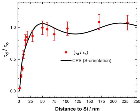
Fig. 4 Normalised phosphorescence lifetime versus distance for the ReC16 monolayer deposited on c-Si. Experimental points are fitted to a modified Chance–Prock–Silbey (CPS, full line) theory with a parallel dipole (S) orientation with QY = 75%.
