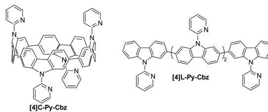
Fig. 1 Molecular structures of tetracarbazole oligomers: cyclic [4]C-Py-Cbz (left) and acyclic [4]L-Py-Cbz (right).
