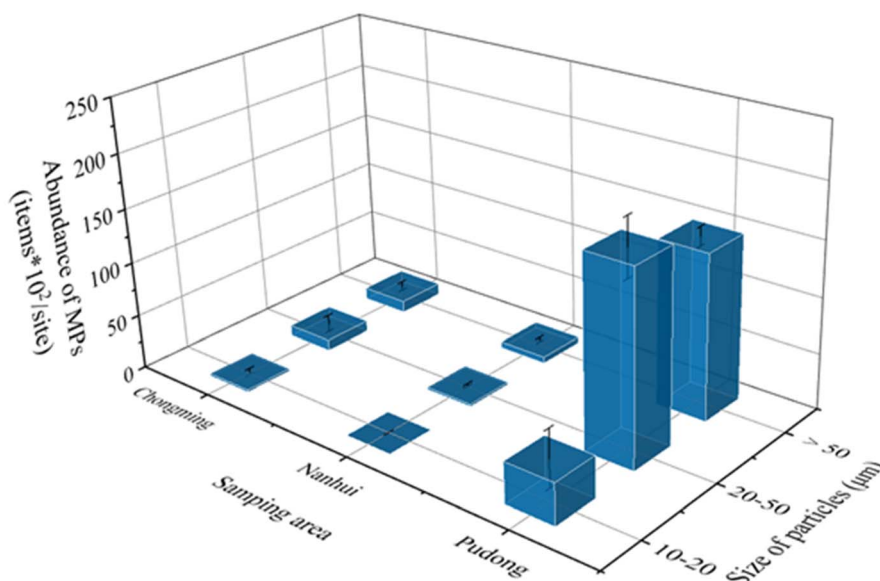
Fig. 7 The characteristics of MPs in the sediment sampling. (A) The morphology and chemical information for MPs in sediment samples with different sizes. Scale bar = 50 \mu\text{m} ; (B) the abundances of MPs with different sizes generated from plastic pieces in different sampling areas.
