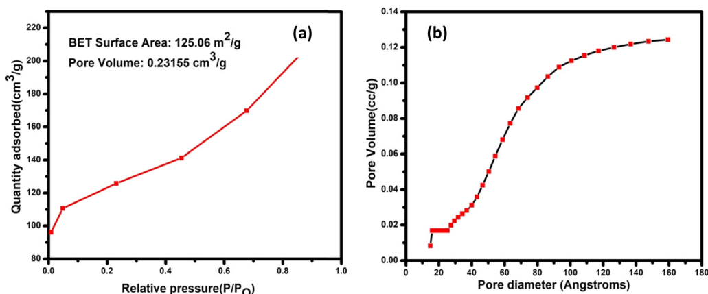
Fig. 4 (a) BET adsorption isotherm and the (b) pore size distribution curve.
