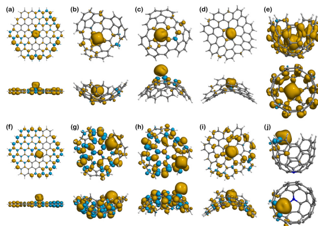
Fig. 8 Spin densities of the \text{Fe(III)} complexes in their most stable spin multiplicity configuration: (a) \text{Fe(III)}@ \text{Planar} ( M = 6 ); (b) \text{Fe(III)}@ \text{Endo} ( M = 5 ); (c) \text{Fe(III)}@ \text{Exo} ( M = 5 ); (d) \text{Fe(III)}@ \text{Negative} ( M = 5 ); (e) \text{Fe(III)}@ \text{Well} ( M = 6 ); (f) \text{Fe(III)}@ \text{N-Planar} ( M = 5 ); (g) \text{Fe(III)}@ \text{N-Endo} ( M = 6 ); (h) \text{Fe(III)}@ \text{N-Exo} ( M = 6 ); (i) \text{Fe(III)}@ \text{N-Negative} ( M = 6 ); (j) \text{Fe(III)}@ \text{N-Well} ( M = 5 ). The yellow density represents the excess of \alpha -electron density. The blue density represents the excess of \beta -electron density.
