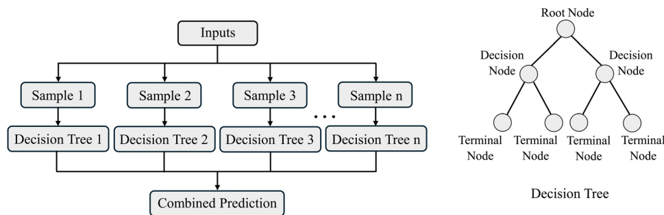
Fig. 4 Random Forest architecture (left) and the base model architecture (right).
