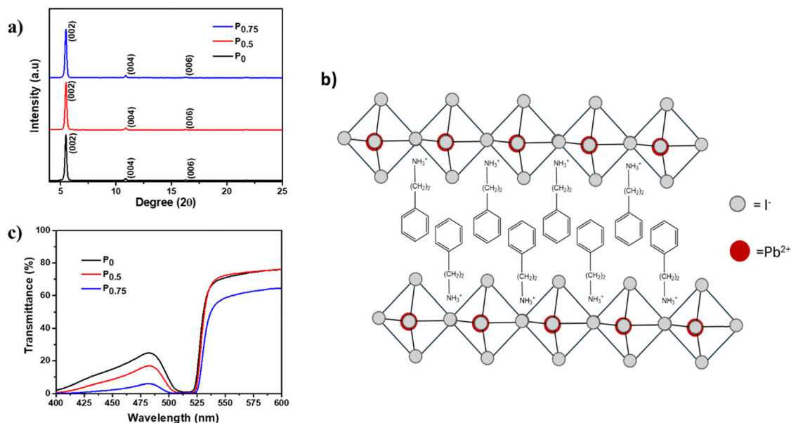
Fig. 1 (a) XRD analysis of P 0 , P 0.5 , and P 0.75 perovskite thin films. (b) Layered structure of the (PEA) 2 PbI 4 perovskite. (c) Transmittance analyses of P 0 , P 0.5 , and P 0.75 compositions. [P 0 = pristine (PEA) 2 PbI 4 , P 0.5 = 0.5 mg PCBM mixed in 1 ml (PEA) 2 PbI 4 perovskite precursor, and P 0.75 = 0.75 mg PCBM mixed in 1 ml (PEA) 2 PbI 4 perovskite precursor solution.]
