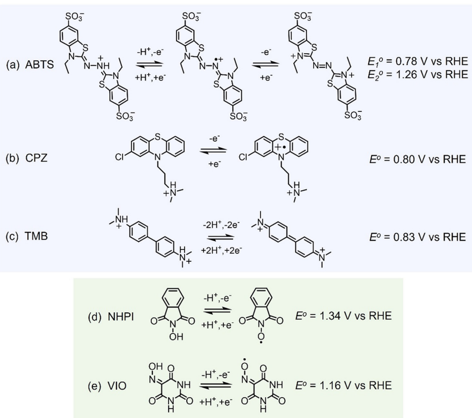
Fig. 5 Determined redox reactions and potentials for (a) 2,2'-azinobis(3-ethylbenzothiazoline-6-sulfonate) (ABTS) in 1 M \text{HClO}_4 , and (b) chlorpromazine (CPZ), (c) N,N,N',N' -tetramethylbenzidine (TMB), (d) N -hydroxyphthalimide (NHPI) and (e) violuric acid (VIO), in 1 M \text{H}_2\text{SO}_4 .
