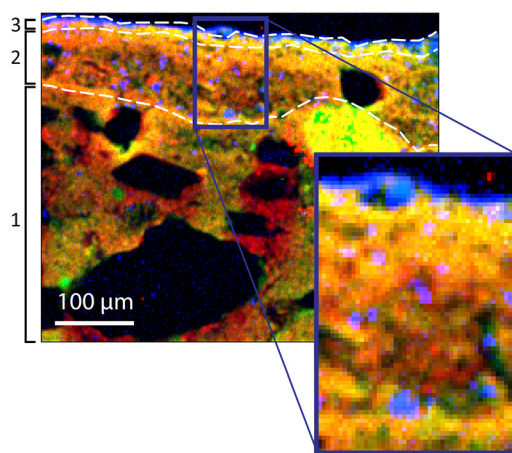
Fig. 6 RGB correlation of the \mu XRD maps of calcite (Cal, red pixels) and of whe-wellite (Whe, blue pixels) together with the \mu XRF maps of calcium (Ca_K, green pixels) in samples S1 and S2. The dotted white lines highlight the layer sequence of the fresco in the two samples.
