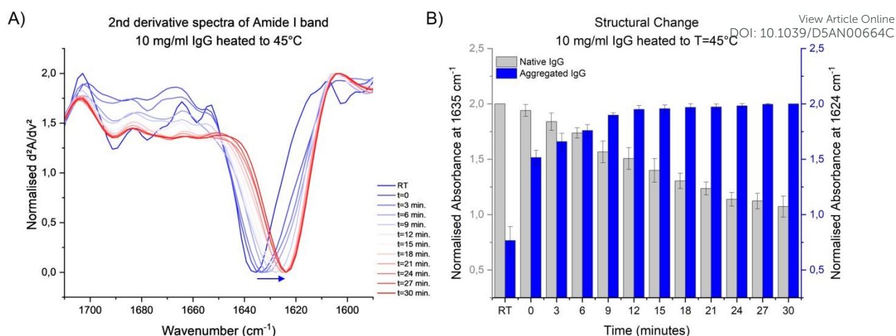
Figure 3. Change in secondary structure of 10 mg/ml IgG in sodium citrate buffer (pH 3.5) during 45 °C flow experiments. A) Normalised second derivative spectra of Amide I band during T=45°C flow experiment, clearly showing a shift in peak position from 1635 cm -1 (intra-molecular beta sheets) to 1624 cm -1 (intermolecular beta sheets); B) Normalised absorbance of second derivative spectra at 1635 cm -1 and 1624 cm -1 over time (n=3). Note that the values plotted in this figure were obtained by flipping the second derivate spectra of Figure 3A around the x-axis and offsetting the spectra by a value of 2. Error bars indicate the standard deviation.
