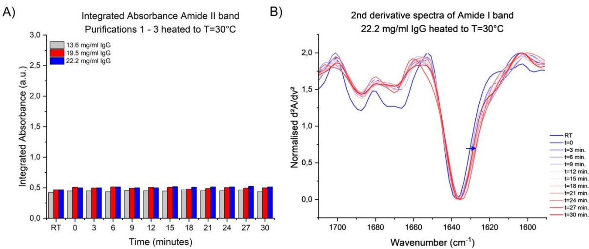
Figure 4. Results of T=30 °C flow experiments with IgG in 0.1 M sodium citrate (pH 3.5) after elution from the protein A column. A) Integrated Amide II absorbance (1580 -1490 cm -1 ) after buffer
