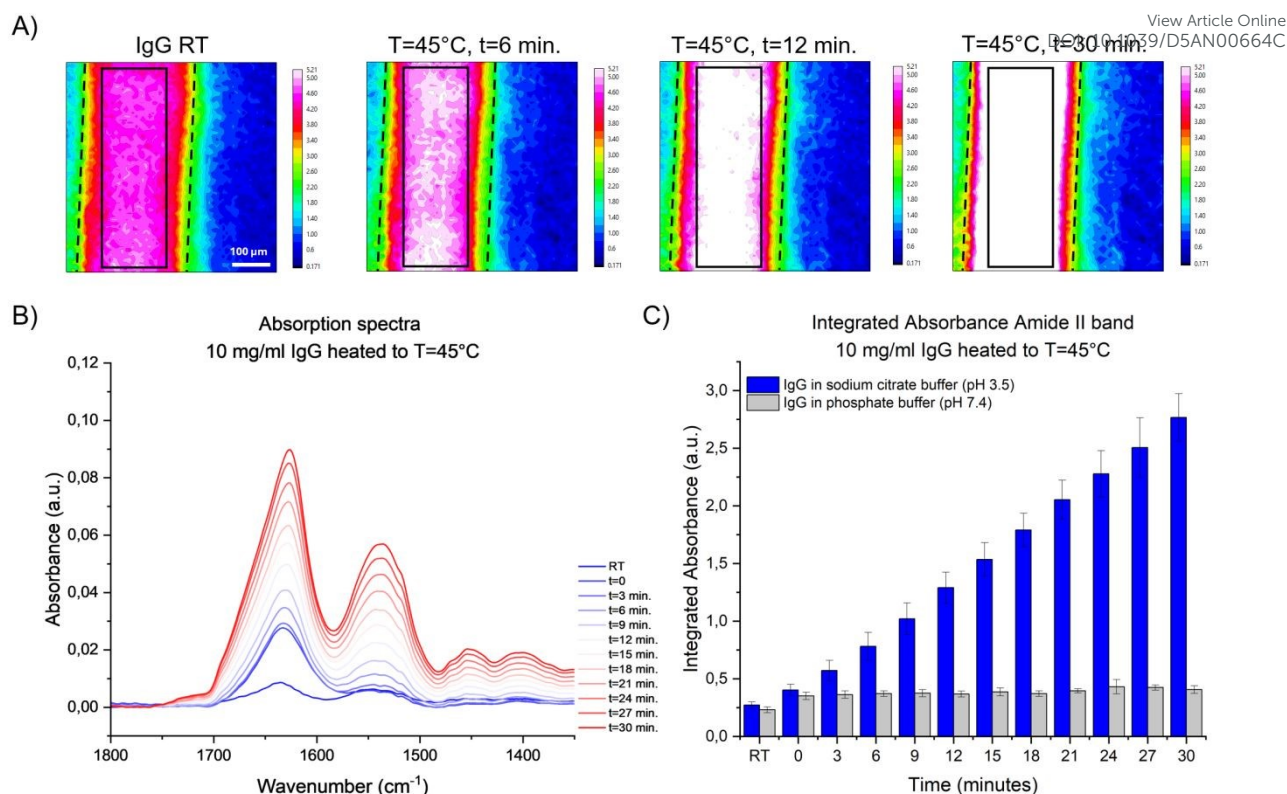
Figure 2. Flow experiments of 10 mg/ml IgG in sodium citrate buffer (pH 3.5) versus phosphate buffer (pH 7.4) at T=45 °C. A) Chemical images of flow channel generated through Amide I band integration (1700 – 1600 \text{cm}^{-1} ), with the black box indicating the area of spectral extraction and the dashed lines indicating the channel wall; B) Buffer-subtracted spectra of IgG in 0.1 M sodium citrate buffer extracted from the flow channel; C) Integrated Amide II absorbance (1580 – 1490 \text{cm}^{-1} ) after buffer subtraction ( n=3 ). Error bars indicate the standard deviation.
