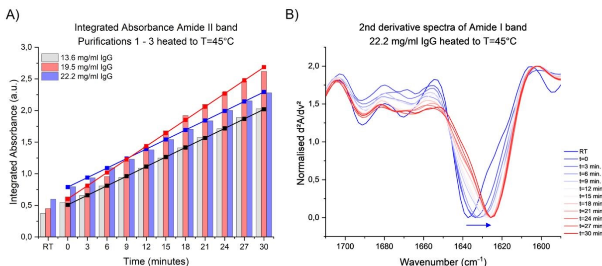
Figure 5. Results of T=45 °C flow experiments with IgG in 0.1 M sodium citrate (pH 3.5) after elution from the protein A column. A) Integrated Amide II absorbance (1580 -1490 cm^{-1} ) after buffer subtraction for samples from purification 1 - 3; B) Second derivative spectra of IgG sample obtained from purification 3 (22.2 mg/ml) at room temperature (RT) and after t=0 to t=30 minutes of heating to T=45 °C.
