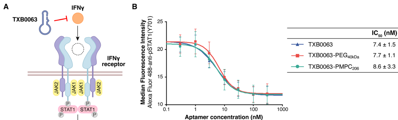
Fig. 3 (A) Inhibitory mechanism of TXB0063 in IFN- \gamma signaling. (B) Inhibition of STAT1 phosphorylation by TXB0063 and TXB0063-polymer conjugates. L929 cells were treated with IFN- \gamma (2 ng mL -1 ) at 37 °C for 15 minutes in the presence of TXB0063 or TXB0063-polymer conjugates. After being washed with ice-cold PBS, the cells were fixed, permeabilized, and immunostained to measure the STAT1(Tyr701) phosphorylation level by flow cytometry. Plotted curves and the median fluorescence intensities are representative of three independent experiments performed in triplicate. IC 50 values are expressed in average \pm standard deviation of the values obtained from each experiment. Inhibition experiments using TXB0063-PTGMA 200 and random oligonucleotide control are shown in Fig. S4.†
