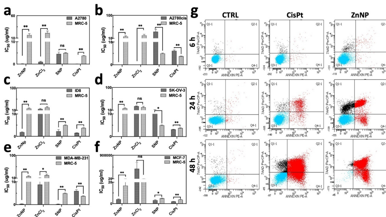
Fig. 3 Evaluation of cytotoxicity. (a–f) IC 50 values of ZnNP toward non-tumoral and tumoral cells. Values are expressed as \mu\text{g ml}^{-1} . (g) Apoptosis analysis. A2780 cells were analyzed by FACS using Annexin V/7AAD double staining after 6, 24 and 48 h treatment of ZnNP ( 50\text{ }\mu\text{g ml}^{-1} ) and CisPt ( 3\text{ }\mu\text{g ml}^{-1} ; 10\text{ }\mu\text{M} ) (Q3: viable cells, Q4: early apoptosis, Q2: late apoptosis, Q1: necrosis). Groups were considered statistically significant if p < 0.05 (*), p < 0.01 (**) and, non-significant (ns). Error bars indicate SD.
