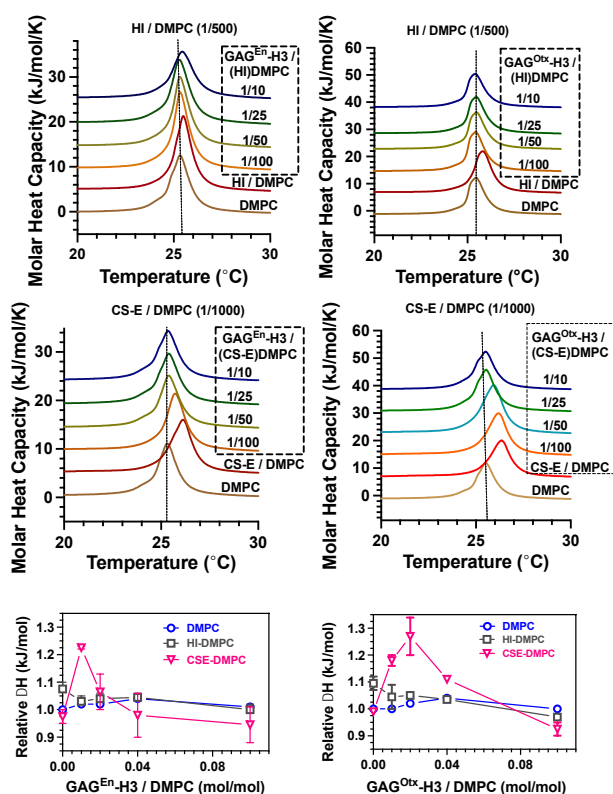
Fig. 6 DSC analysis of enthalpy changes upon addition of GAG En -H3 (a, b, c) or GAG Otx -H3 (d, e, f) to 1 mg/mL HI- (grey) or CS-E-decorated (pink) DMPC LUVs in HEPES buffer plus Ca 2+ , Mg 2+ . (c, f) Curves correspond to the relative \Delta H that is the ratio between the enthalpy recorded with GAG-decorated DMPC LUVs and the one with pure DMPC LUVs (blue), according to different ratios of peptide / DMPC LUVs.
