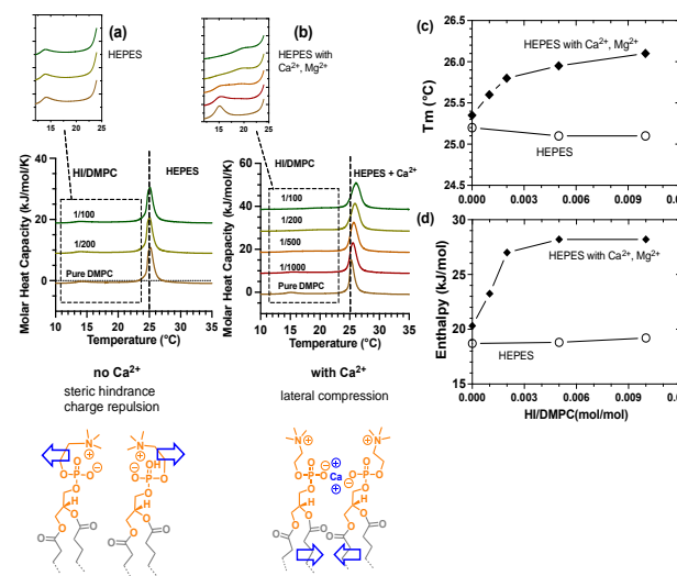
Fig. 5 DSC analysis of T_m and enthalpy changes upon addition of heparin (HI) to 1 mg/ml DMPC LUVs in (a) HEPES buffer and (b) HEPES buffer plus Ca 2+ , Mg 2+ . Curves correspond to DMPC mixed with different amounts of HI. The pre-transition of DMPC is circled by the dashed rectangle and zoomed in the left top; corresponding main phase transition temperature (c) and enthalpy (d) of DMPC LUVs according to HI/DMPC ratio. The thermograms are from one experiment repeated once. Similar results with DPPC and DSPC in SI. Below thermograms (a) and (b) is represented the hypothesis for the impact of Ca 2+ on PC organization: in the absence of Ca 2+ , the positively charged choline interacts with the negative phosphate moiety of the polar head, which would create steric hindrance or charge repulsion between the polar head groups of adjacent phospholipids; in the presence of Ca 2+ , the divalent ion bridging phosphate moieties would allow the choline headgroup to reorientate outside the bilayer and induce lateral compression between adjacent alkyl chains.
