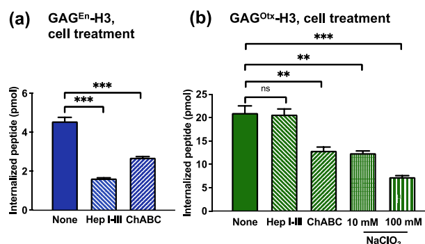
Fig. 4 MALDI-TOF MS quantification of internalized (pmol) chimeric peptides incubated (7 \mu M) 1 hr at 37°C with one million SKOV-3 cells submitted to GAG hydrolysis (HepI-III, ChABC) or desulfation (NaClO 3 ).
