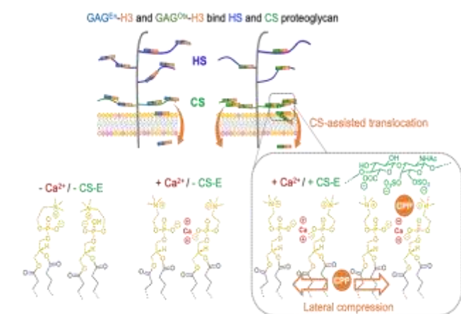
Fig. 8 Schematic representation of the proposed role of GAGs in the internalization mechanism of the chimeric peptides studied herein: GAG OTx and GAG En , H3 and chimeric GAG OTx -H3 and GAG En -H3. CS are located at the vicinity of the lipid bilayer while HS are more distal. The chimeric CPPs bind to HS- and CS- proteoglycans. (CS-E bind PC lipids in the presence of \text{Ca}^{2+} , leading to an overall anionic complex. Therefore, there are no longer repulsion forces between the cationic choline headgroup and the cationic peptide, could then insert deeper into the lipid bilayer to cross it.
