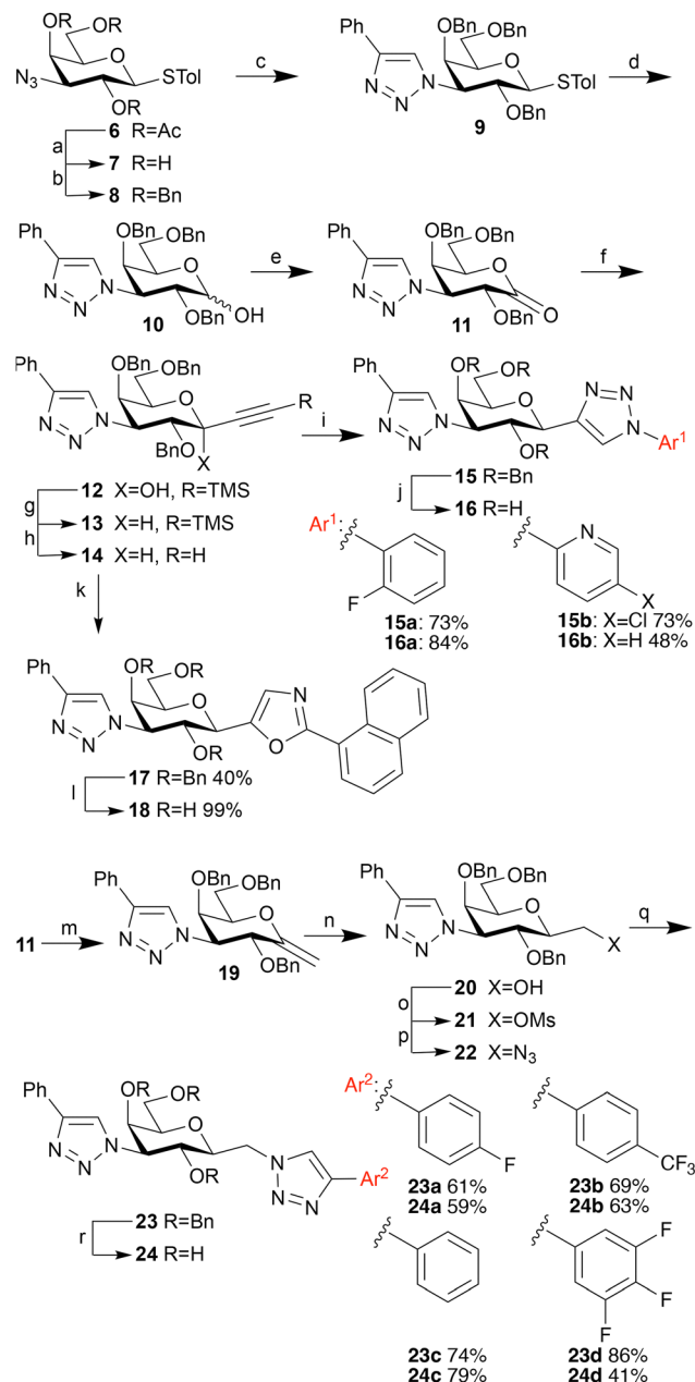
Scheme 2 Synthesis of 1,3-dideoxy-1-(aryltriazolyl)-3-(phenyltriazolyl)- \beta -D-galactopyranosides 15a–b , 1,3-dideoxy-1-(1-naphthyltriazolyl)-3-(phenyltriazolyl)- \beta -D-galactopyranoside 17 and 1-deoxy-3-(phenyltriazolyl)-1-(aryltriazolyl)-methyl- \beta -D-galactopyranosides 24a–d . (a) Sodium methoxide, methanol (dry), r.t., 2 h, 95%. (b) Sodium hydride, benzyl bromide, THF (dry), reflux 18 h, 84%. (c) Phenylacetylene, copper(i) iodide, triethylamine, ACN (dry), r.t., 18 h, 84%. (d) N -Bromosuccinimide, acetone/water, r.t., 10 min, 92%. (e) Dess–Martin periodinane, DCM (dry), r.t., 18 h, 99%. (f) Cerium(III) dichloride trimethylsilyl acetylde, THF (dry), -78^{\circ}\text{C} to r.t., 8 h, 78%. (g) Triethylsilane, boron trifluoride etherate, ACN/DCM (dry) 0^{\circ}\text{C} , 8 h, 60%. (h) Tetrabutylammonium fluoride, THF, r.t., 10 min, 91%. (i) Aryl azide, Copper(i) iodide, triethylamine, ACN (dry), r.t., 18 h. (j) Palladium hydroxide on carbon, cyclohexene/ethanol, reflux. (k) 1-Cyanonaphthalene, [Bis(trifluoromethanesulfonyl)imidate] (triphenylphosphine)gold(i), 8-methylquinoline N -oxide, 55^{\circ}\text{C} , sealed tube under nitrogen. (l) Palladium hydroxide on carbon, cyclohexene/ethanol, reflux. (m) Petasis reagent, toluene, 80^{\circ}\text{C} , 48 h, 63%. (n) Borane dimethyl sulfide, THF (dry), 0^{\circ}\text{C} , 12 h, then hydrogen peroxide, sodium hydroxide, THF/water, 0^{\circ}\text{C} , 2 h, 62%. Diastereoselectivity 4:1 \beta : \alpha . (o) Mesyl chloride, pyridine, 0^{\circ}\text{C} , 2 h, 95%. (p) Sodium azide, DMF (dry), 95^{\circ}\text{C} , 2 h, 92%. (q) Aryl acetylene, copper(i) iodide, triethylamine, ACN (dry), r.t., 18 h. (r) Palladium hydroxide on carbon, cyclohexene/ethanol, 80^{\circ}\text{C} , 18 h.
