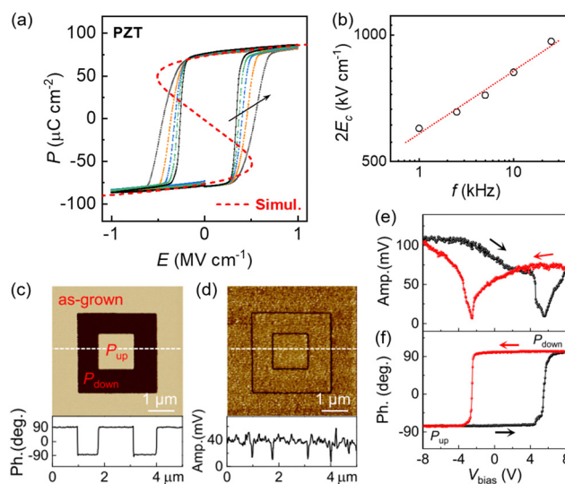
Fig. 4 Ferroelectric properties of PZT thin films. (a) P – E loops at different V bias frequencies, and (b) 2E c vs. f for an Au/100 nm PZT/10 nm LaNiO 3 capacitor on STO. Reproduced from ref. 39 with permission from American Physical Society, copyright 2021. (c)–(f) PFM studies of a 50 nm PZT/10 nm LSMO heterostructure on STO. (c) PFM phase and (d) amplitude images of concentric square domains. (e) PFM amplitude and (f) phase switching hysteresis. Reproduced from ref. 48 with permission from American Physical Society, copyright 2021.
